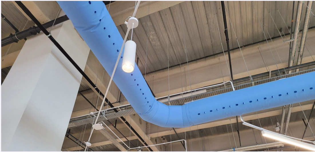
Figure 8. Textile air distribution ducts applied in a building.
